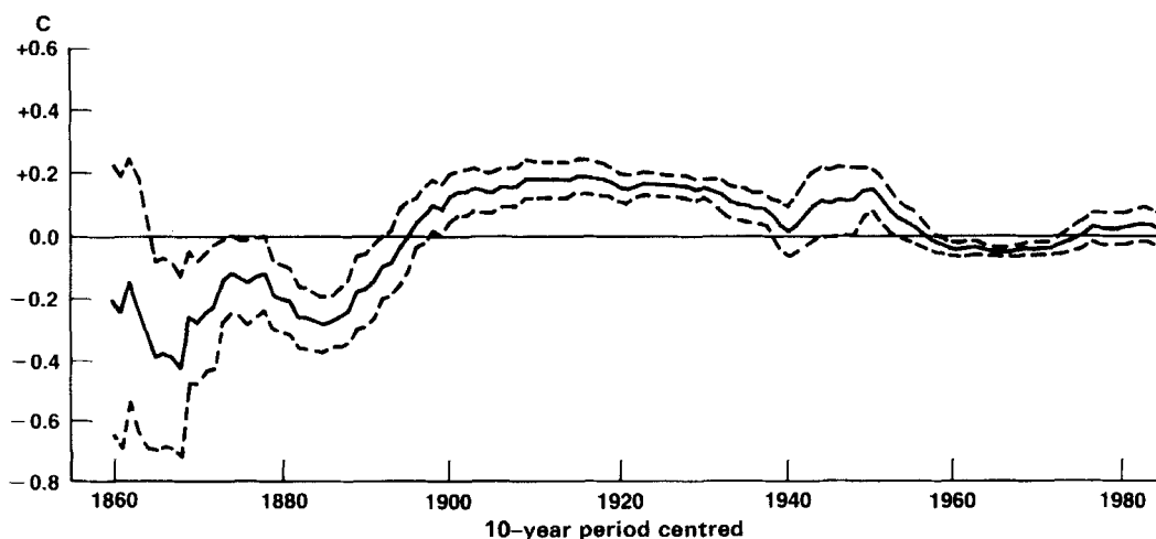
Figure 15. Ten-year running mean differences (solid line) between coastal and island air temperatures and nearby sea-surface temperatures for the tropics (20°N–20°S), relative to 1951–1980. The dashed lines are \pm two standard errors estimated from the variability of the differences between sites. Land data were provided by P. D. Jones, University of East Anglia © HMSO
