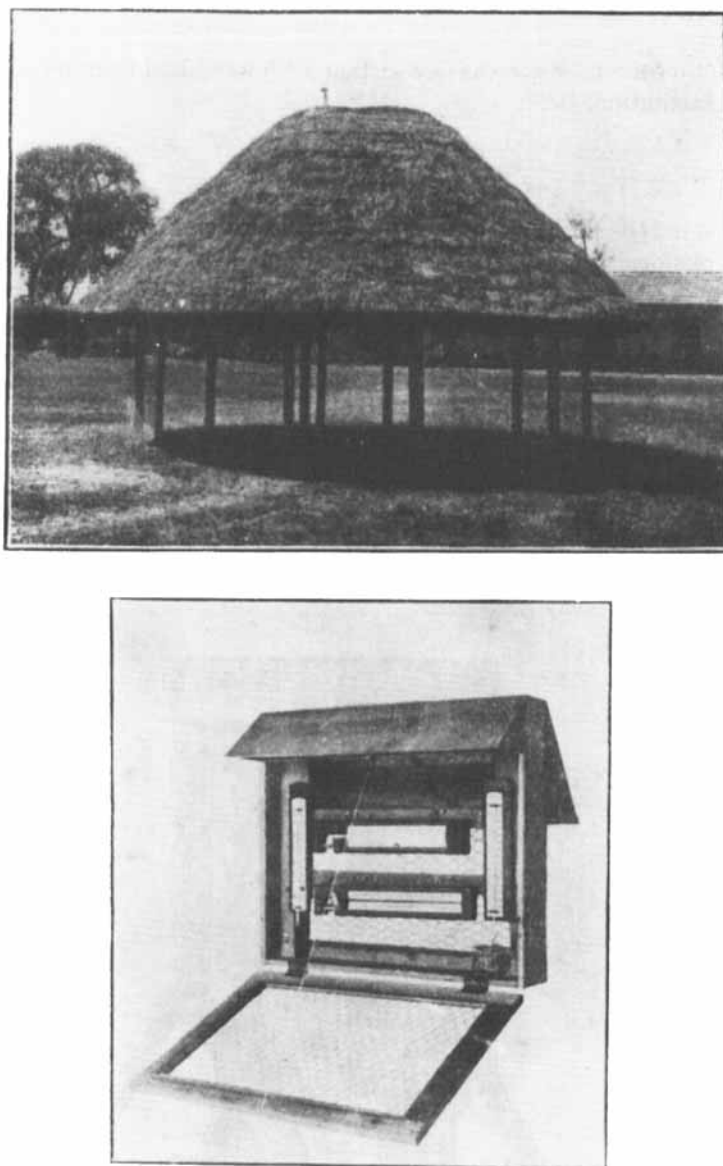
Figure 4. Thatched shelter and associated thermometer cage for use in the tropics (from Field, 1920) © HMSO
